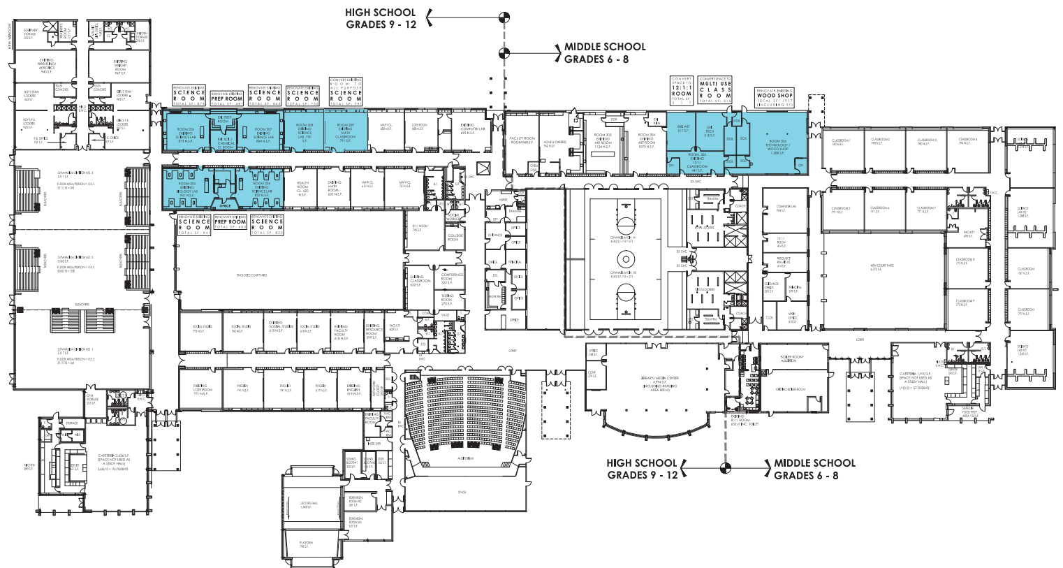
PROPOSED FIRST FLOOR PLAN CENTER MORICHES HIGH SCHOOL
